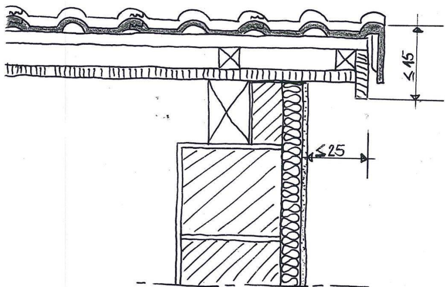
SKIZZE ORTGANG
